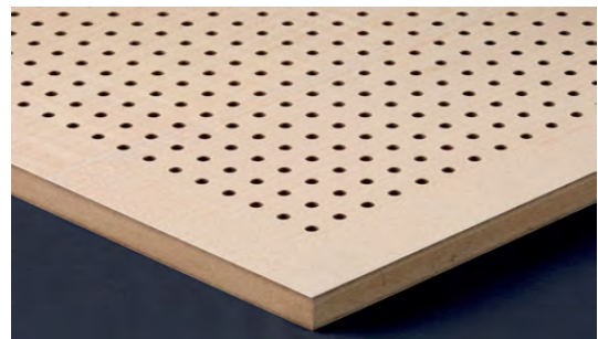
Typ: 3-8 ( \phi = 3 mm, Achsabstand = 8/16+32 mm)
